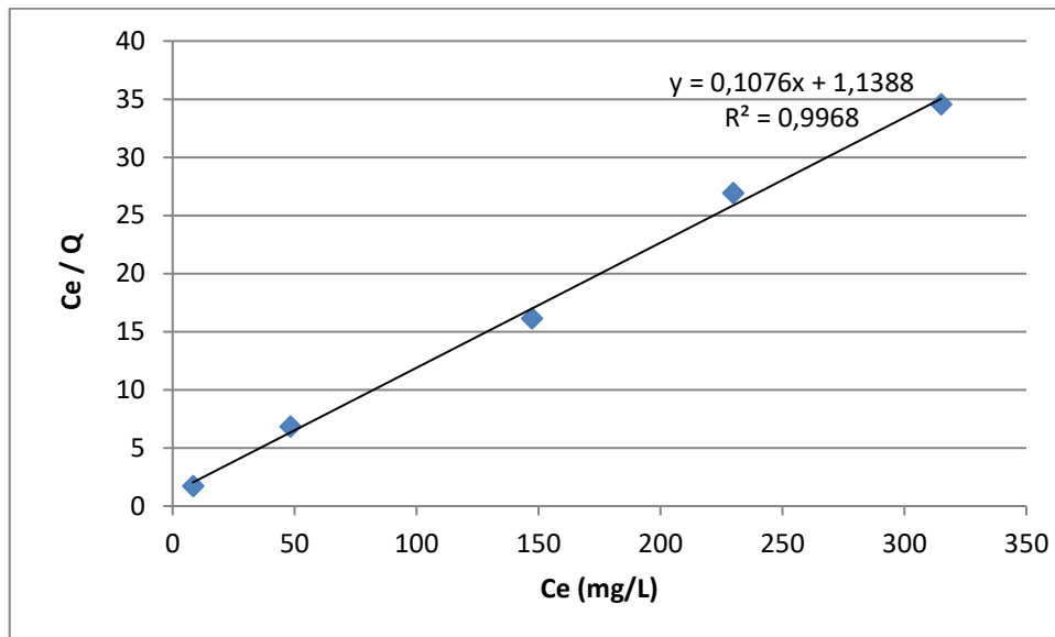
Gambar 7. Grafik Adsorpsi Isotermal Langmuir
